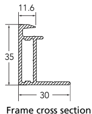
Frame cross section
